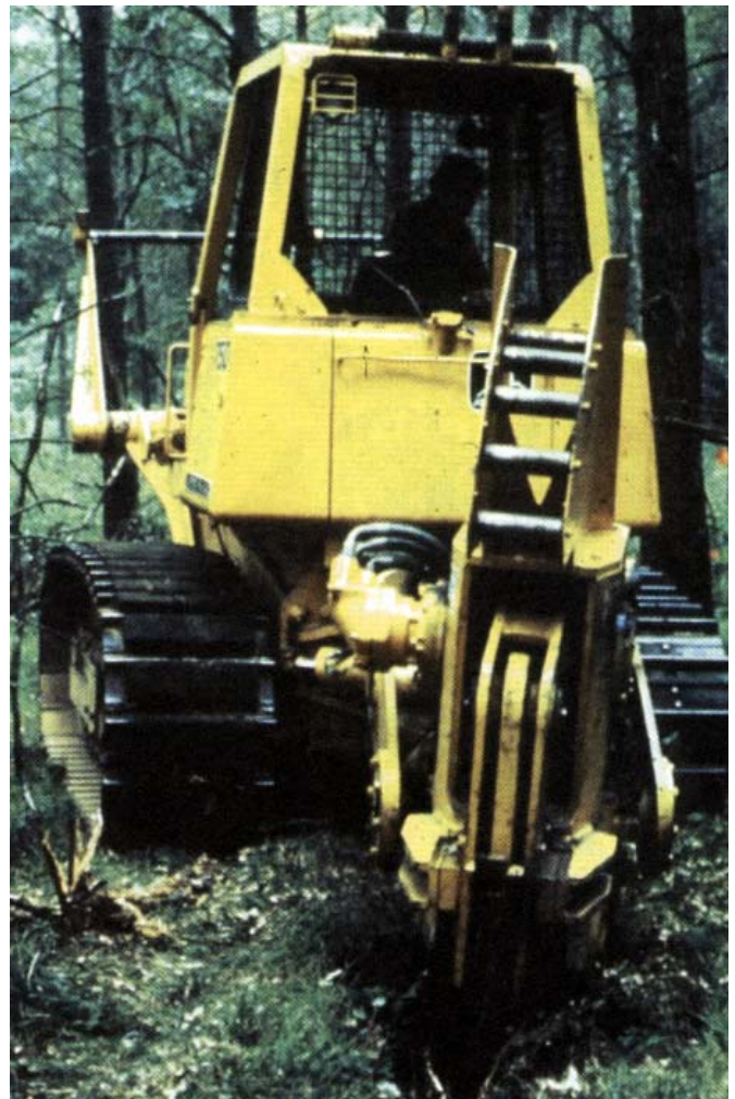
Figure 10 A vibratory plow with a 5-foot blade is most effective in severing root grafts between infected and healthy oak trees in locations where no underground pipes or cables are buried.
